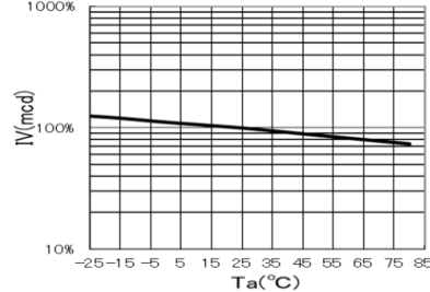
◆ IV-Ta Characteristics (YG) IF=20mA
