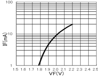
◆ IF-VF Characteristics (YG)
