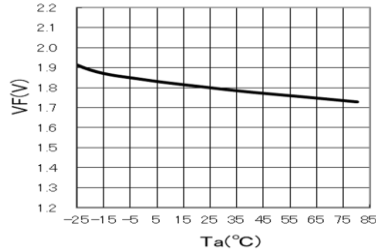
◆ IV-Ta Characteristics (HR) IF=20mA
