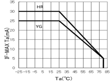
◆ IF-Max Ta Characteristics
