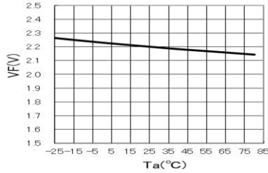
◆ IV-Ta Characteristics (YG) IF=20mA
