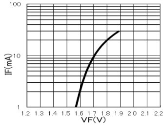
◆ IF-VF Characteristics (HR)
