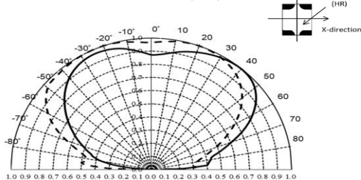
◆ Directive Characteristics (HR)
