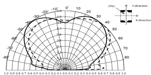
◆ Directive Characteristics (YG)
