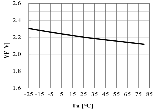
◆ IV-Ta Characteristics
