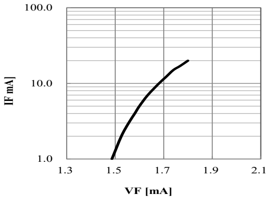
◆ IV-IF Characteristics
