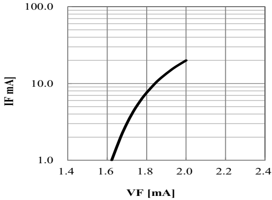
◆ IV-IF Characteristics
