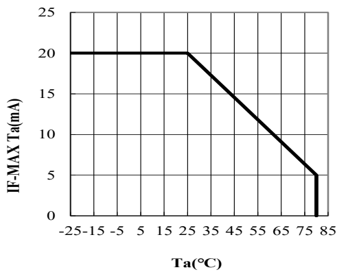
◆ IF-Max Ta Characteristics
