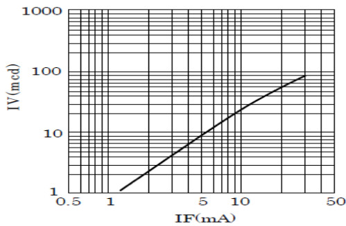
◆ IV-IF Characteristics
