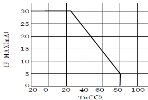
◆ IF-Max Ta Characteristics
