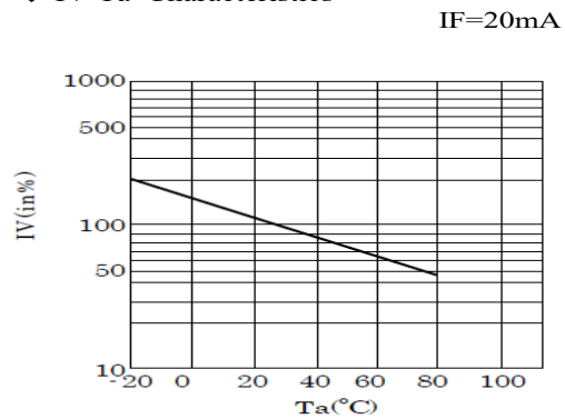
◆ IV-Ta Characteristics
