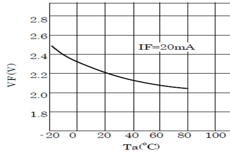
◆ VF-Ta Characteristics
