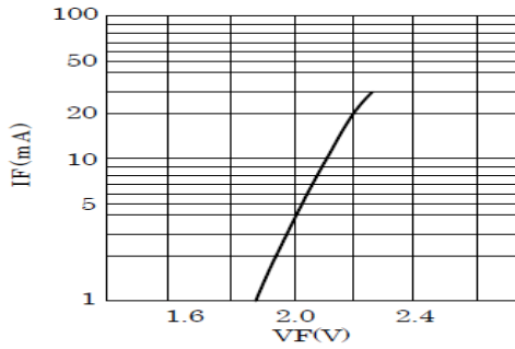
◆ IF-VF Characteristics
