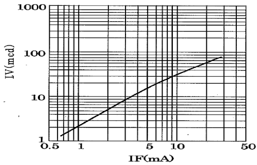
◆ IV-IF Characteristics
