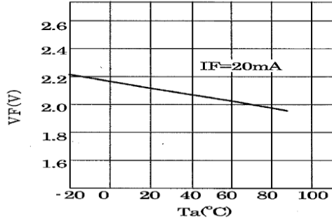
◆ VF-Ta Characteristics
