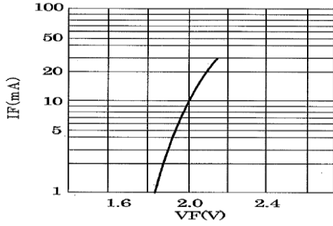
◆ IF-VF Characteristics
