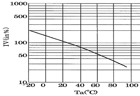
◆ IV-Ta Characteristics
