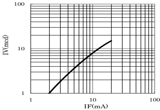
◆ IV-IF Characteristics
