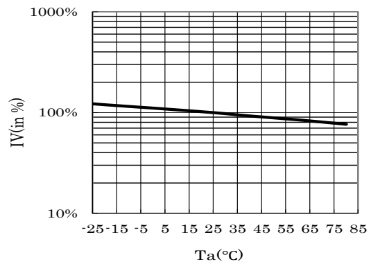
◆ IV-Ta Characteristics
