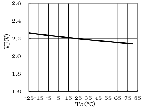
◆ IV-Ta Characteristics
