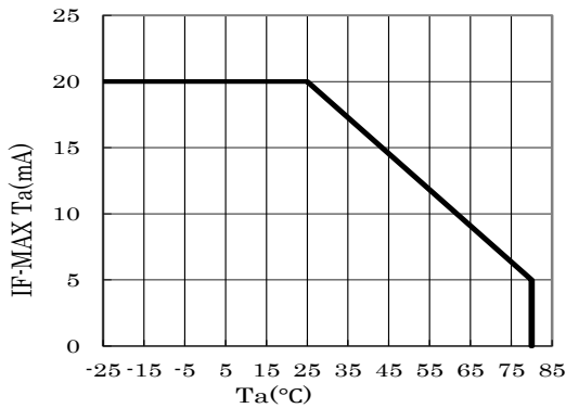
◆ IF-MAX Ta Characteristics
