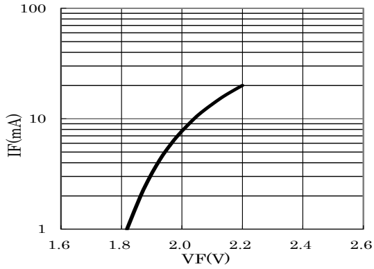
◆ IV-IF Characteristics
