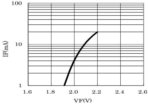
◆ IV-IF Characteristics
