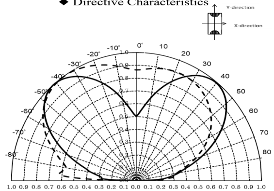
◆ Directive Characteristics
