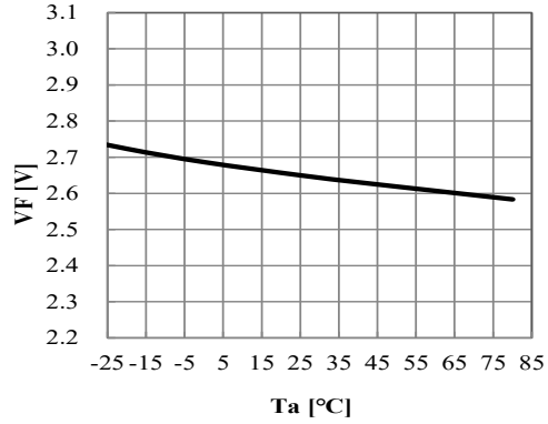
◆ IV-Ta Characteristics
