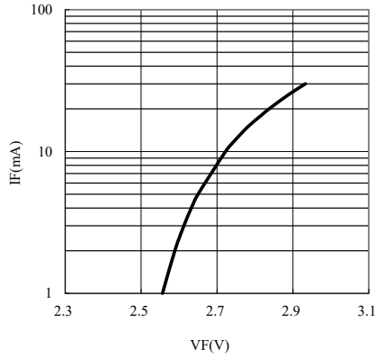
◆ IV-IF Characteristics
