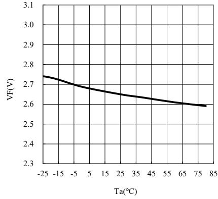
◆ VF-Ta Characteristics IF=20mA
