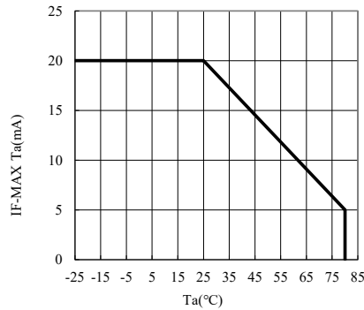
◆ IF-MAX Ta Characteristics (Blue)
