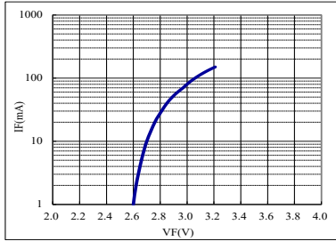
◆ IV-IF Characteristics
