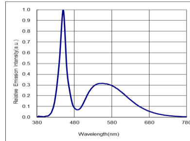
◆ Spectral Distribution
