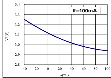
◆ VF-Ta Characteristics
