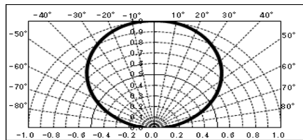
◆ Directive Characteristics
