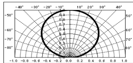
◆ Directive Characteristics
