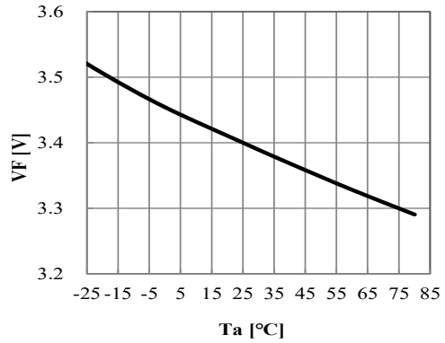
◆ IV-Ta Characteristics
