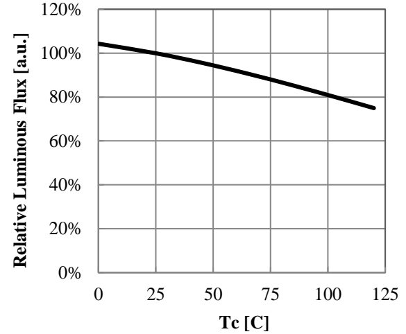
Case Temperature vs. Relative Luminous Flux If=700mA
