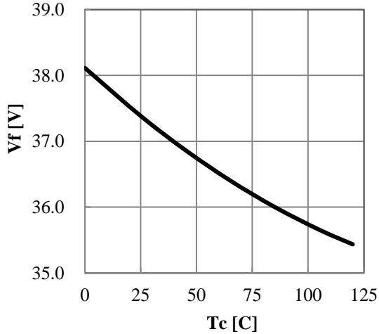
Case Temperature vs. Forward Voltage If=700mA
