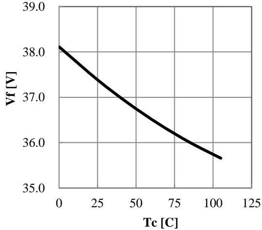
Case Temperature vs. Forward Voltage If=1050mA
