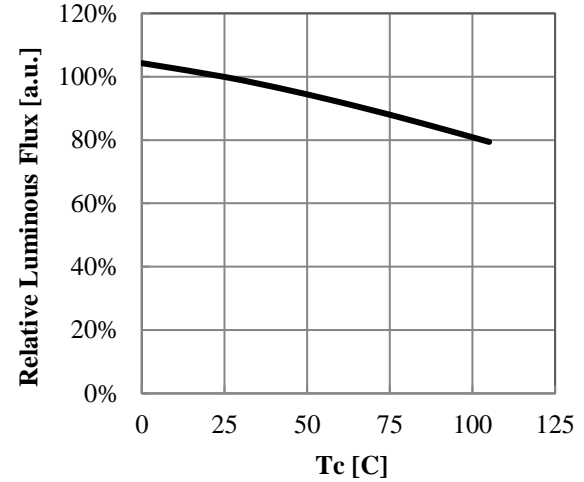
Case Temperature vs. Relative Luminous Flux If=1050mA
