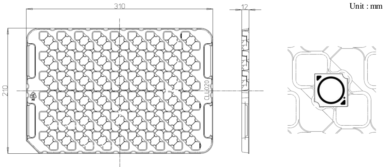
Product 54 pcs/tray
