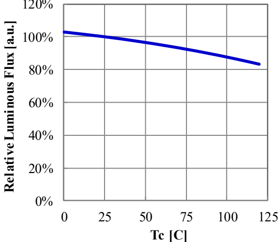
Case Temperature vs. Relative Luminous Flux If=900mA
