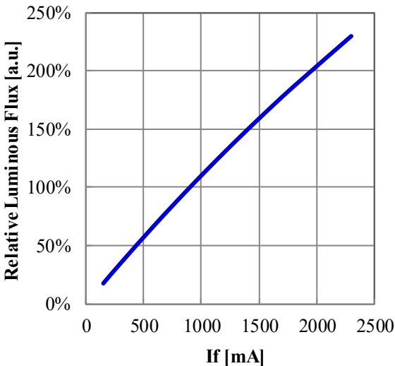
Forward Current vs. Relative Luminous Flux Tc=25C
