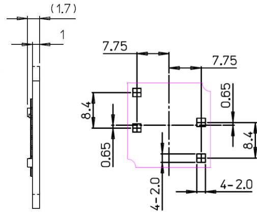
PAD position layout
