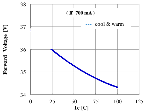
Case Temperature vs. Forward Voltage
