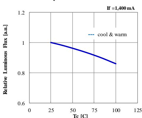
Case Temperature vs. Relative Luminous Flux
