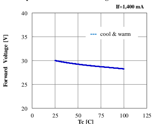
Case Temperature vs. Forward Voltage
