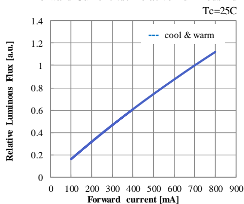
Forward Current vs. Relative Luminous flux
