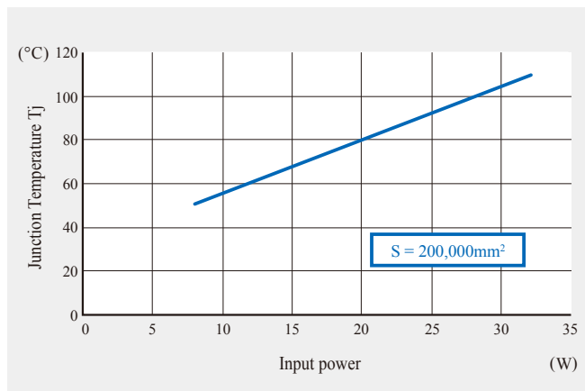
Figure-3 ( b ) Input power - junction temperature T_j (CLU034-1205B8)
