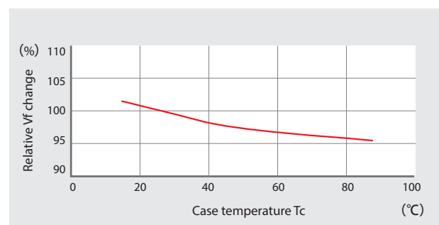
■ 図2 Tc -Vf characteristic
