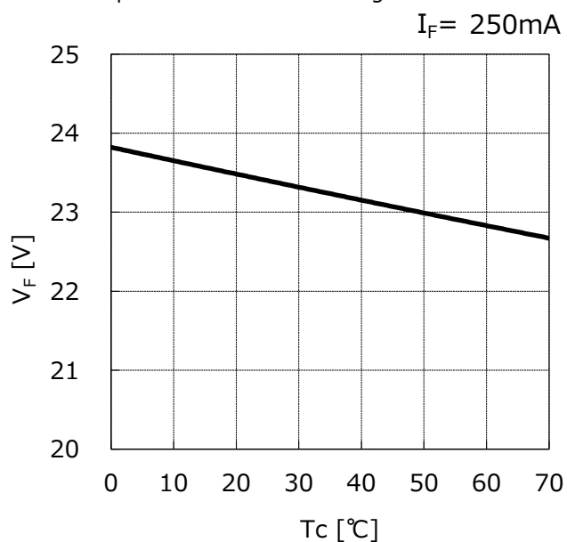
◆ T c Temperature – Forward Voltage Characteristics
