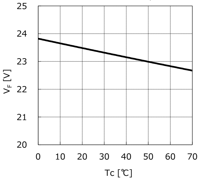
◆ T c Temperature – Forward Voltage Characteristics I F = 250mA
