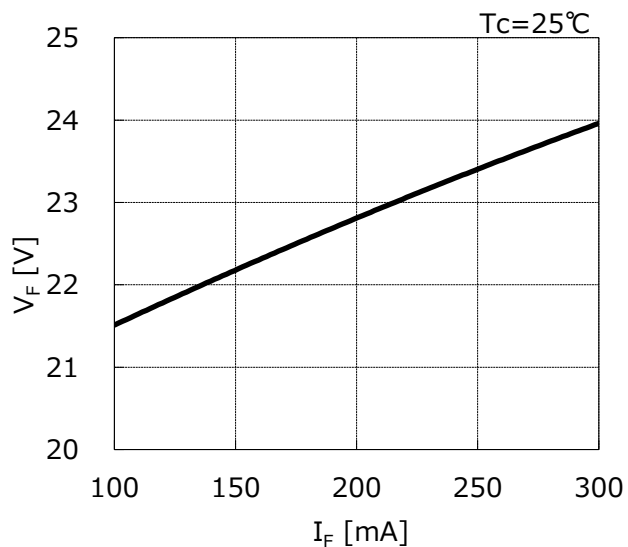
◆ Forward Current – Forward Voltage Characteristics
