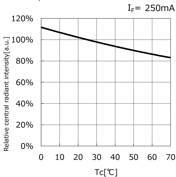
◆ T c Temperature – Relative Central radiant intensity
