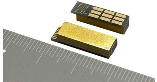
W5.0 × D17.5 × H3.3 mm
